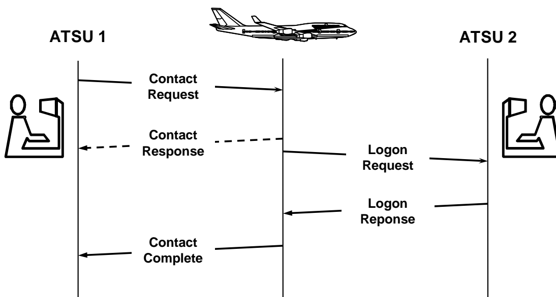
Figure 2-8. Air-ground address forwarding message sequence (Transfer between areas where data link is provided)
